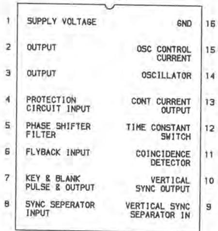
IC401 TDA1180P
