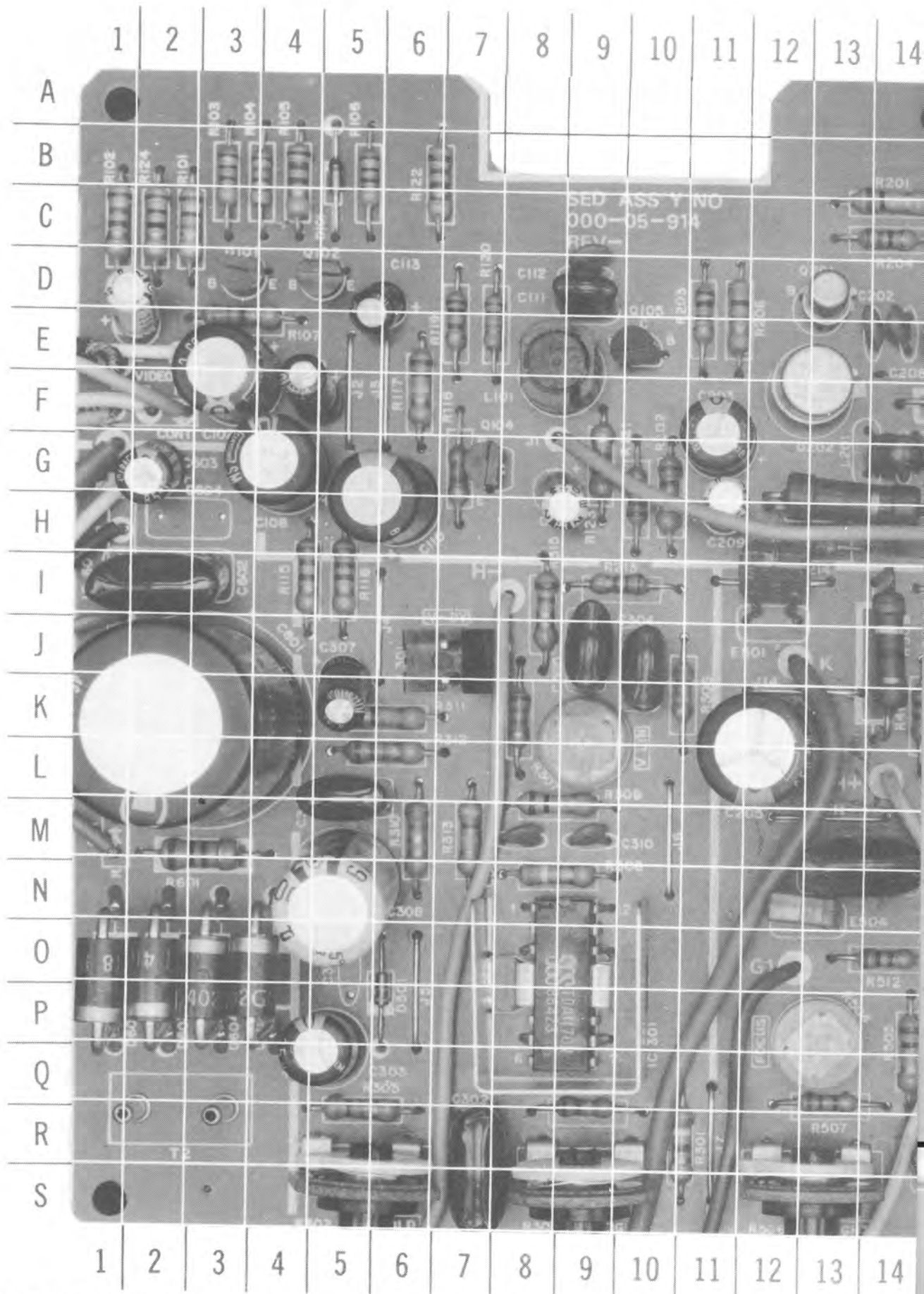
MAIN BOARD 060-01-001 REV B
