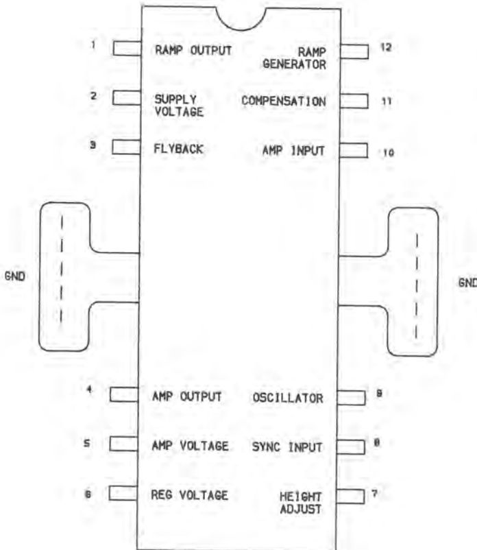
IC301 TDA1170N
